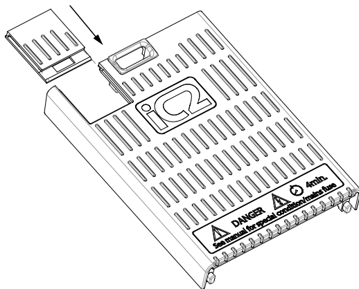
Illustration 12: Installing the Sliding Door
